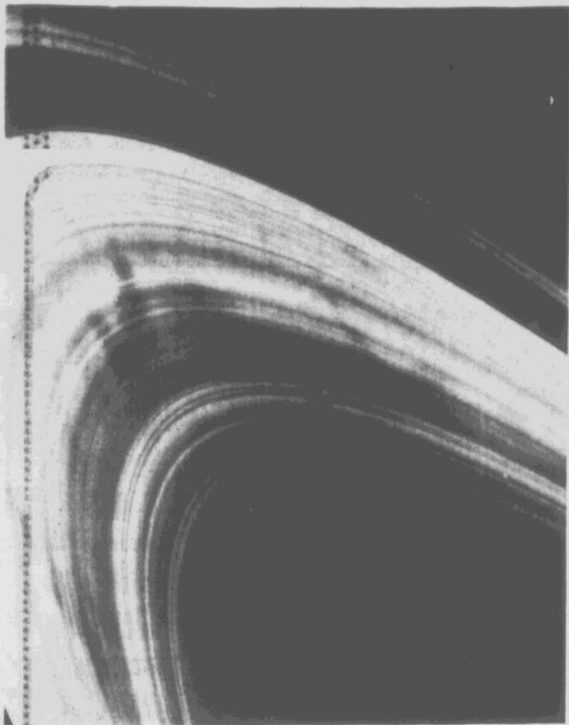
SPOKE FEATURES — Voyager II obtained this high-resolution picture of Saturn's rings on August 22 from a distance of 2.5 million miles. Evident are the numerous "spoke" features in the B-ring: their very sharp, narrow appearance suggests short formation times. Scientists think electromagnetic forces are responsible in some way for these features, but no detailed theory has been worked out. (AP Laserphoto)
