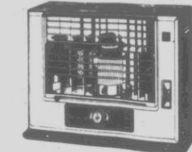
RADIANT 36™ Rated at 9,600 BTUs per hour. Offers sleek designer styling and a removable fuel canister for extra easy filling—a great convenience. Operates up to 25 hours on 1.3 gals. kerosene. 17" high; 25 1/4" wide; 12 1/4" deep. 25.3 Lbs.
