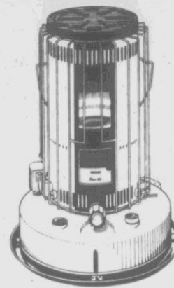
Omni 105™ Rated at a tremendous 19,500 BTUs per hour for biggest heating jobs—cold basements, garages, adjoining rooms, warehouses, barns, construction sites. Operates up to 18 hours on 1.99 gals. kerosene. 22" high; 18 1/2" base. 26.4 lbs. U.L. Listed.
