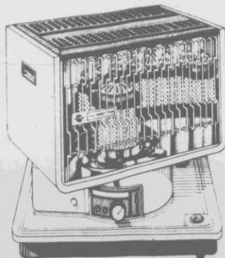
THE DIRECTOR™ Highest rated radiant model, with a unique rotating head to direct heat where you want it. Rated at 11,700 BTUs. Operates up to 32 hours on 1.99 gals. of kerosene. 19 7/8" high; 21 3/4" wide; 19 3/8" deep. 35.2 Lbs. U.L. Listed.
