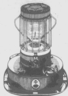
Moonlighter™ Most versatile heater gives heat and light, plus cooking surface. Rated at 8,700 BTUs per hour. Creates a pretty prism-effect. Cookrill and other accessories available. Operates up to 36 hours on 1.7 gals. kerosene. 16 1/2" high; 16 1/4" base. 14.1 lbs. U.L. Listed.
