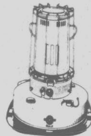
OMNI 15™ Rated at 8,700 BTUs per hour. Smallest lowest-priced Kero-Sun is extra tough for camping or around the house. Offers cooking surface. Operates up to 36 hours on 1.7 gals. kerosene: 15 1/8" high; 16 1/4" base. 14.1 Lbs. U.L. Listed.
