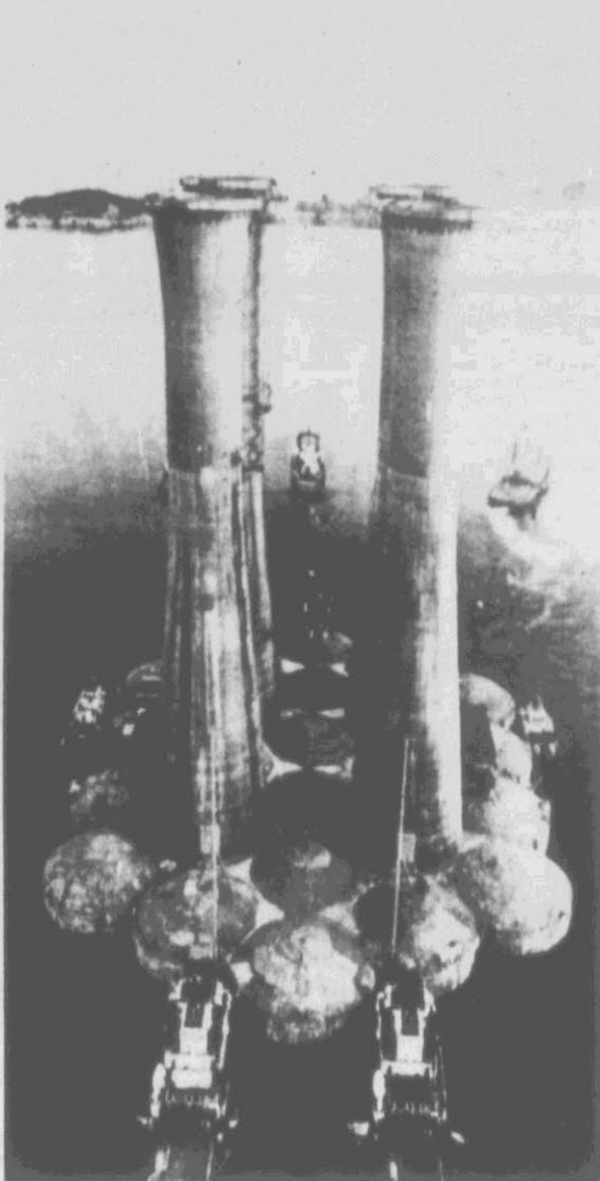
WORLD'S BIGGEST — A 657,000-ton concrete structure is towed from Stavanger for the Norwegian Stratford B offshore oil platform recently. When fully completed with a steel deck attached on top of the 585-foot base, the offshore platform will be about 895 feet tall from top to bottom, and weigh 816,000 displacement tons, the biggest in the world for its kind. (AP Laserphoto)
