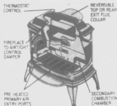
The Wood-Burning VIGILANT
