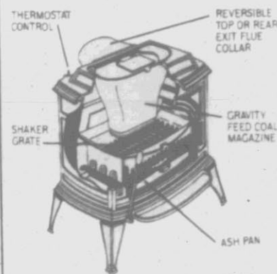
The Coal-Burning VIGILANT "Our stove within a stove"
