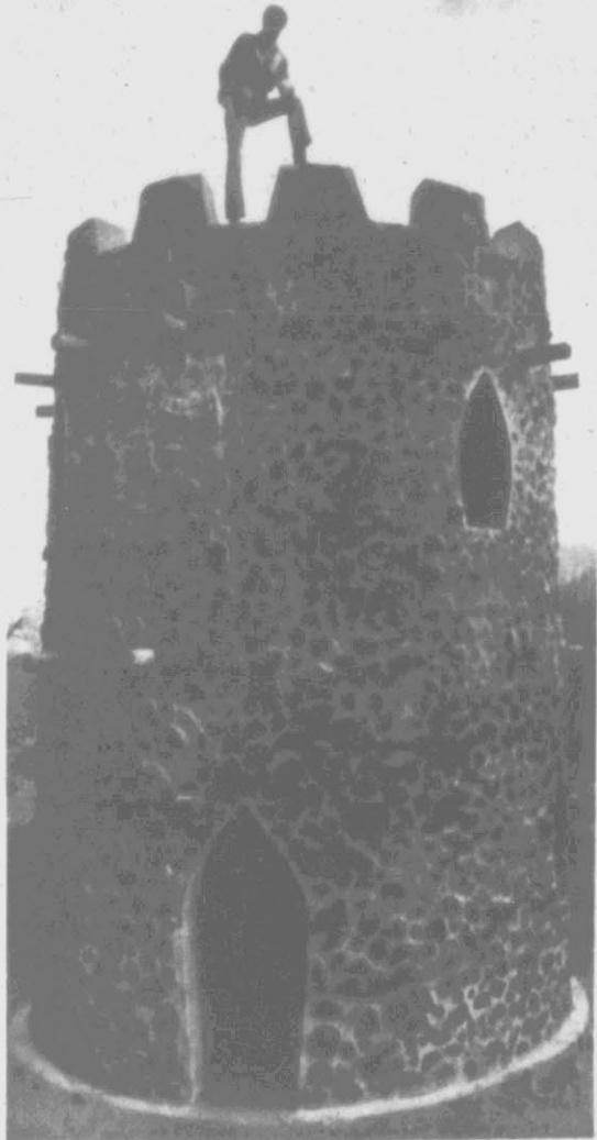
CORDWOOD CASTLE — Ben Flemming stands atop a cordwood castle built as one of the seminar projects of the Mother Earth News magazine, based in Hendersonville, N.C. It is made with firewood logs, placed so only their ends show and surrounded by mortar. (AP Laserphoto)
