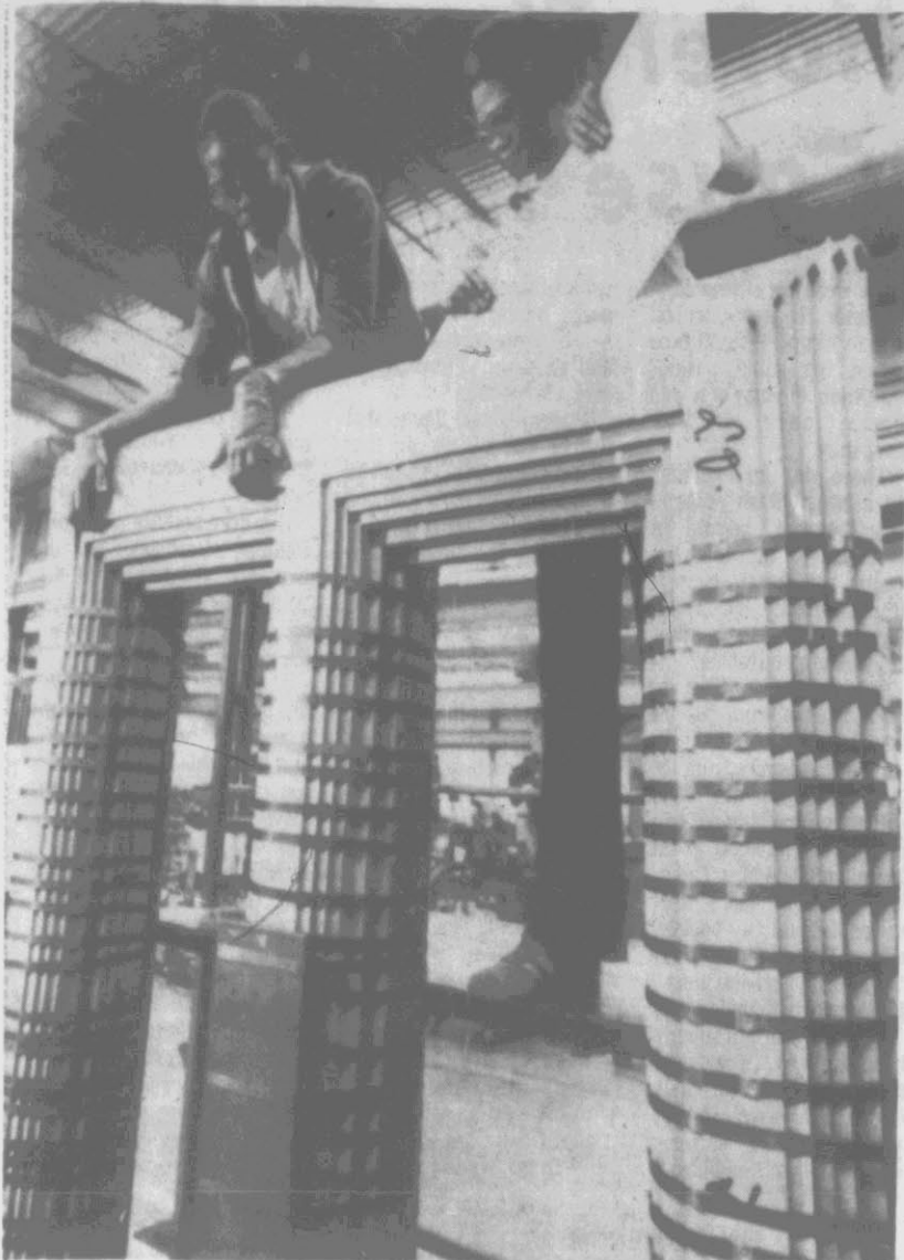
TRANSFORMED STACKS — Precision sheared silicon steel plates are stacked by technicians Annie Williams, right, and Keith Harrod at the GTE Electrical Equipment transformer plant in Hampton, Va. The plates, when fully assembled, will form the core of a Sylvania dry-type transformer with an environmentally safe, vacuum cast, solid epoxy coil. These transformers are an alternative to PCB-filled, liquid-type transformers which were recently banned by the federal government. (AP Laserphoto)
