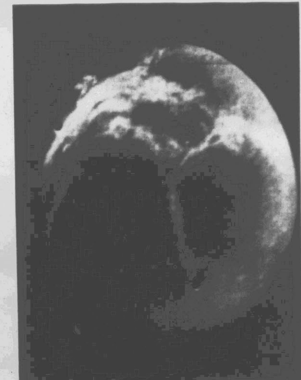
SATURN'S MOON DIONE — Circular craters can be seen in this image taken by Voyager I of Saturn's moon Dione from 790,000 kilometers (500,000 miles). The icy moon surface is only 11 kilometers (700 miles), and the markings on the moon are slightly brighter than the brightest features seen by Voyager on Jupiter's moons, suggesting that they are surface frost deposits. (AP Laserphoto)
