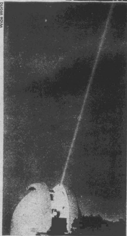
Above, a telescopic view of the heavens. Left, the nine-foot telescope at the University of Texas' McDonald Observatory fires a beam of light skyward in an attempt to measure the distance between the earth and the moon.
