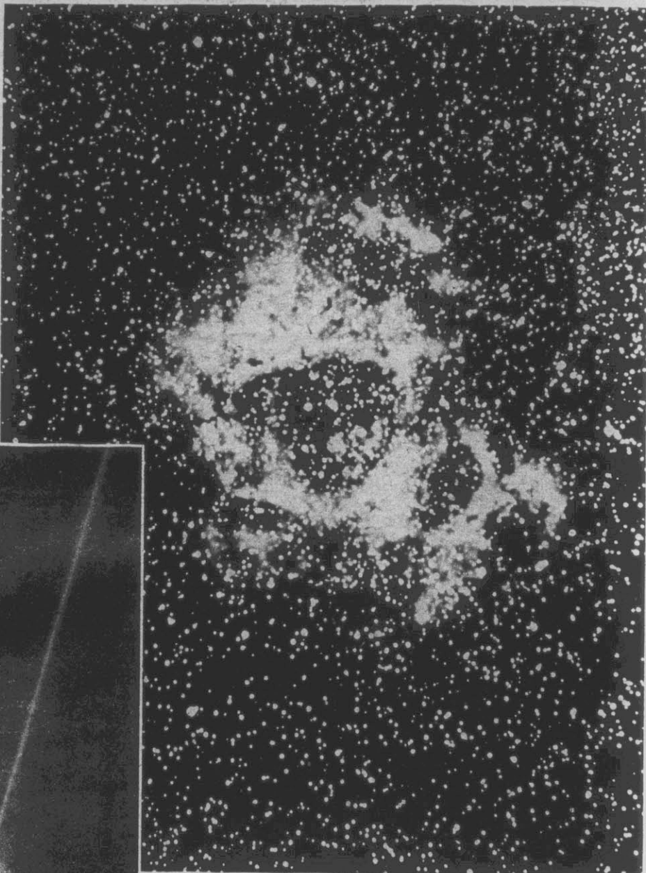
Above, a telescopic view of the heavens. Left, the nine-foot telescope at the University of Texas' McDonald Observatory fires a beam of light skyward in an attempt to measure the distance between the earth and the moon.
