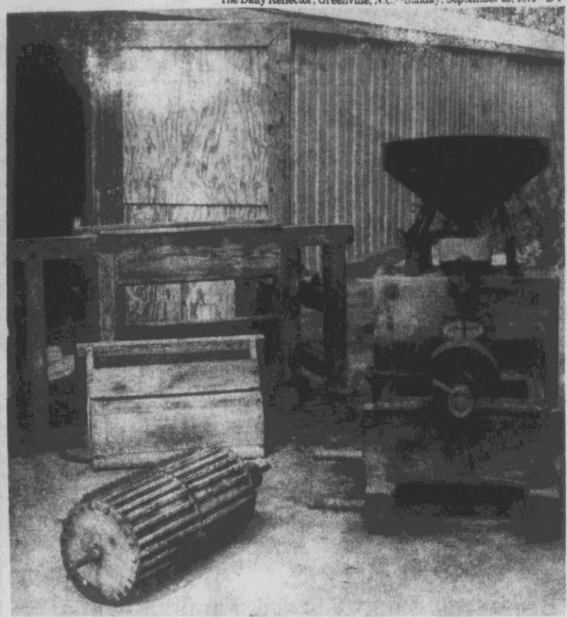
TWO PRIZED ITEMS . . . A 40-saw cotton gin, dating about 1856, is shown in three sections (at left). At the right is a corn and feed grinding mill of the early 1900s.
