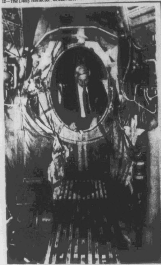
AREA OF STRESS — Fred Lind, vice-president of maintenance for Eastern Airlines, examines the aft bulkhead in a DC-9 for evidence of stress in Miami. Lind is shown on the passenger's side of the bulkhead. The federal government has ordered all DC-9s inspected after an Air Canada plane lost its tail cone in flight. Eastern has 62 DC-9s in its fleet and has completed the inspection on most of them. (AP Laserphoto)
