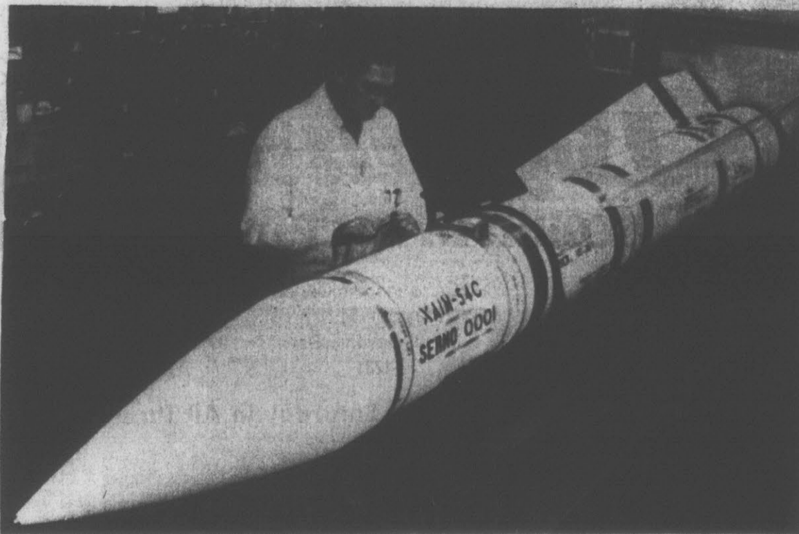
IMPROVED PHOENIX — A technician at Hughes Aircraft Company's Missile systems Group in Canoga Park, Calif., makes final adjustments on the first engineering development model (EDM-1) of the improved Navy AIM-54C Phoenix air-to-air
