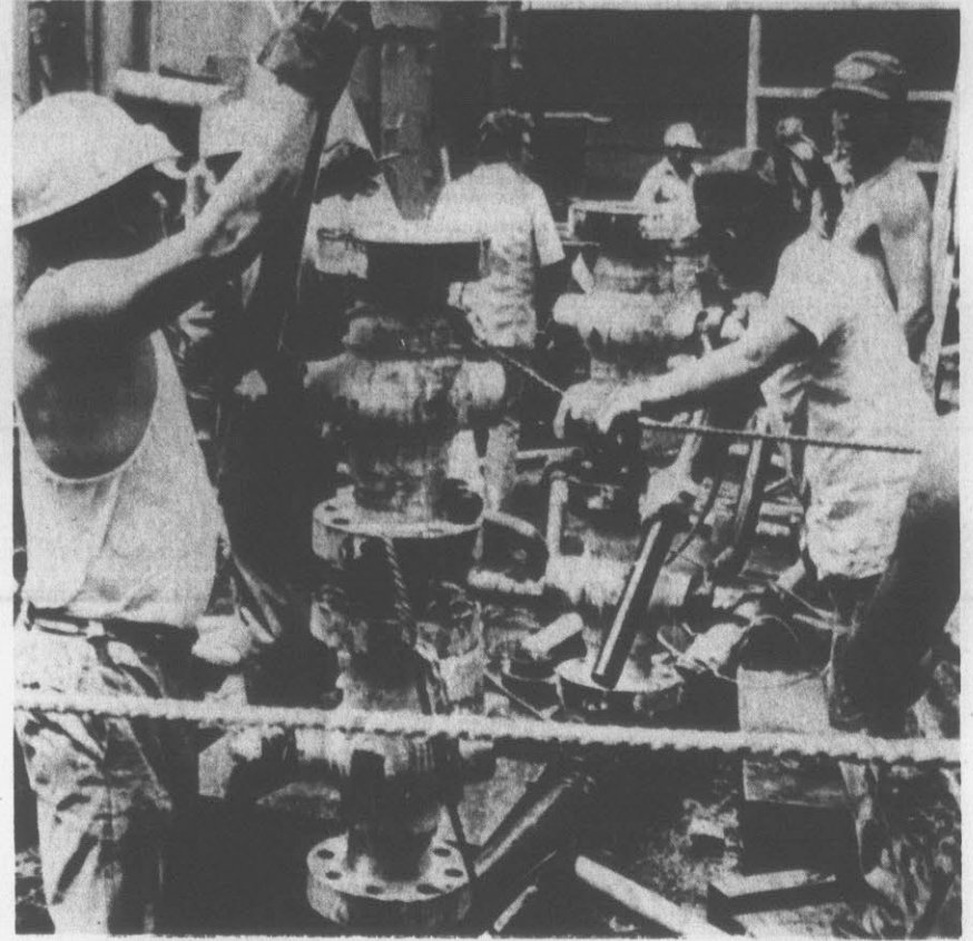
TRYING TO TAME A RUNAWAY WELL — Workmen aboard the ship L.B. Meaders use special equipment to force steel and lead balls in a gelatin-like mixture down the runaway Ixtoc 1 oil well in the Bay of Campeche to try to
