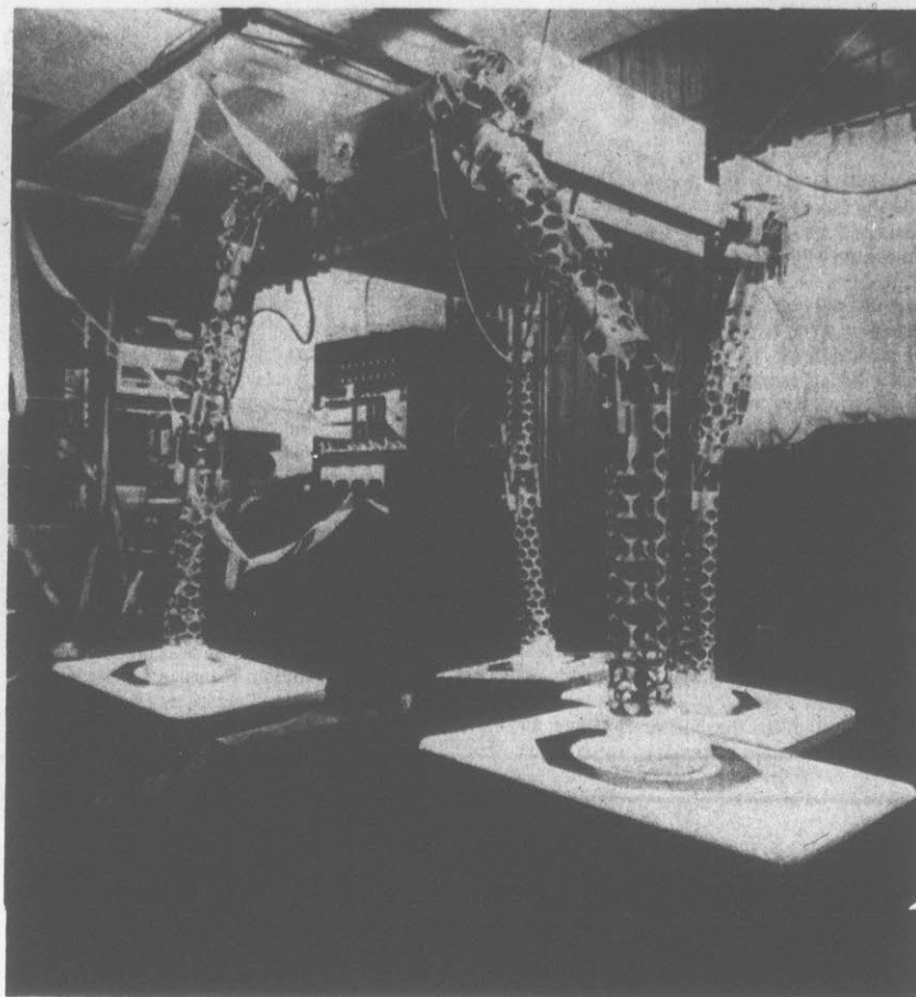
A SERVIPEDE TO NAVY — This is a machine invented by Andrew Weisberg, which no longer exists except as parts in the Lawrence Laboratories at Livermore, Calif. The government calls it a "Rigid Jointed Limbed Vehicle for Walking on Water With Flanged Feet." The Navy calls it a servipepe and the inventor calls it a mechapod. AP Laserphoto
