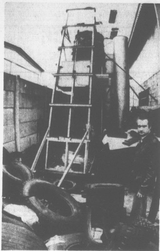
OIL OUT OF RUBBISH — Italian industrialist Andrea Rossi, 28, stands in front of his plant making oil out of rubbish, including old tires, on the outskirts of Milan. His plant processes ten tons of rubbish daily, obtaining two tons of good oil, six tons of coal and two tons of gas. According to the inventor, on an industrial basis the process could be very cheap. Also, in view of the expected Middle East oil shortage, it could solve at the same time the big problem of the elimination of urban solid wastes. (AP Laserphoto)
