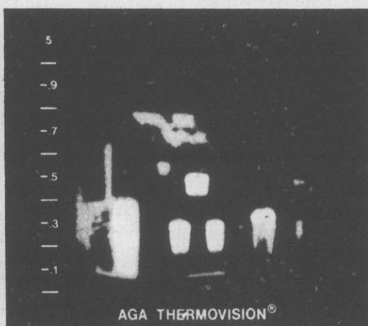
A Thermogram, or "heat loss picture" of the model house clearly shows the defects. The whiter, or lighter-colored areas show where heat-and energy dollars—are being wasted.
