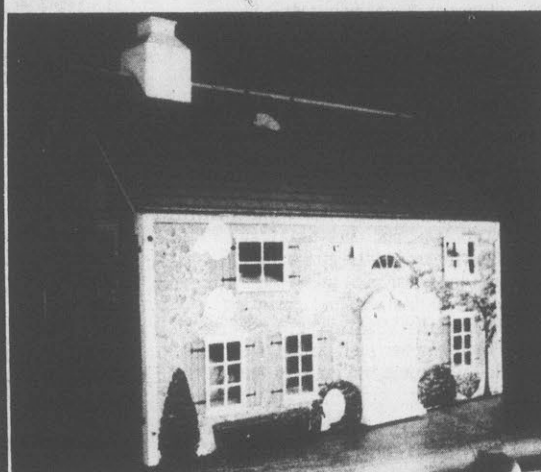
A model house specially built to contain construction defects, such as missing insulation and cold air infiltration problems which can't be seen.
