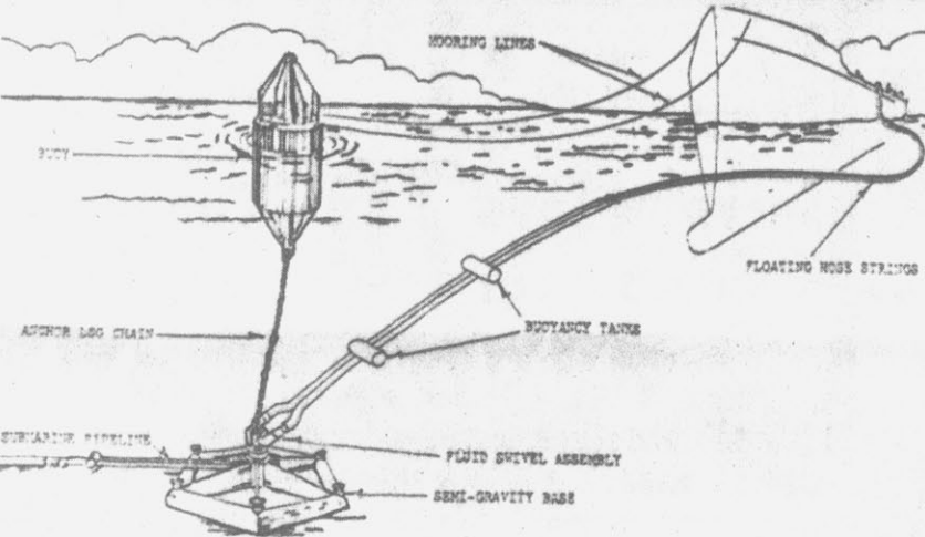
OFFSHORE OIL PORT — Construction of the Louisiana Offshore Oil Port will begin this month with completion due in 1980. It will be the only port in the U.S. large enough to hold supertankers longer than four football fields. Part of the system will employ a mooring buoy (bottom sketch) able to unload crude oil in manner shown in top photo of a tanker unloading abroad, using a similar facility. (UPI Photo)
