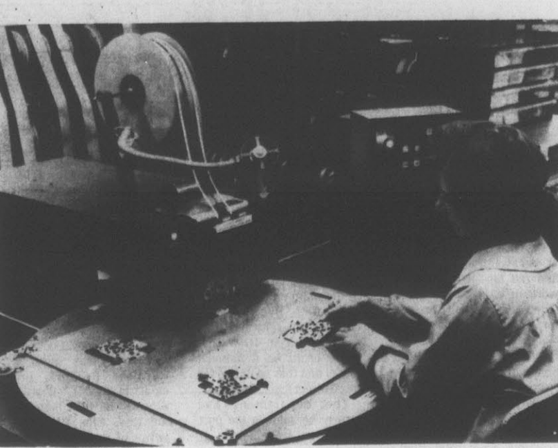
COMPUTERIZED ASSEMBLY — Rose Marie Parascenzo sits at a rotating table that is part of a computer-controlled machine that assembles a single circuit board in one-fifth the time required for manual assembly. This unit
