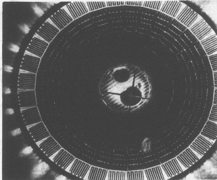
SPACE TANK — Engineers inspect the inside of a 500,000-gallon space shuttle external tank being built at the National Aeronautics and Space Administration's Michoud assembly plant in New
