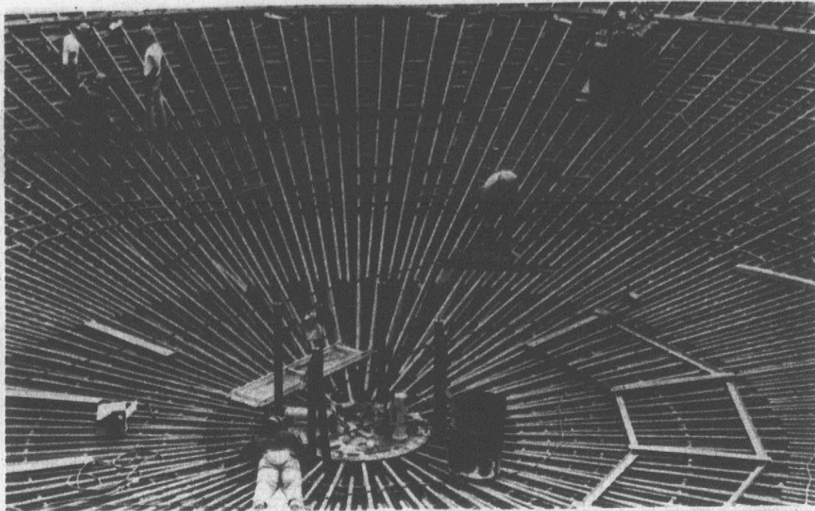
SPIDERMEN — Construction workers appear to be suspended in reinforcing steel used in one of four nuclear reactors under construction at the Hartsville (Tenn.) nuclear plant. An estimated 60,000 tons of steel bars like these will be used in 3.5 billion dollar
