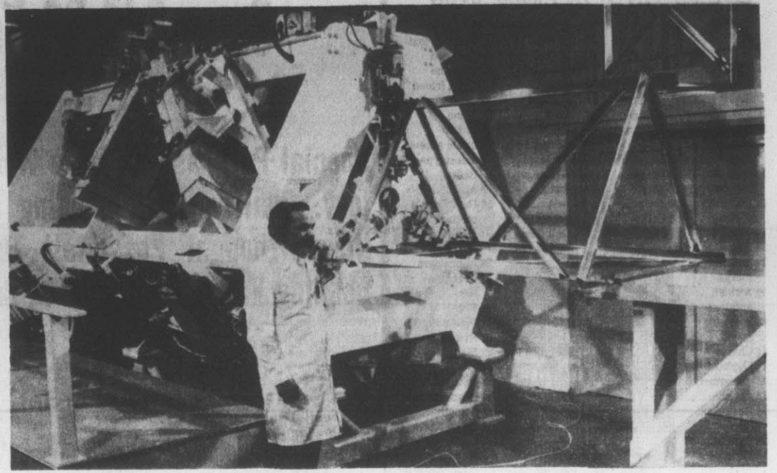
OUTER SPACE CONSTRUCTION — Bill Boucher, an electronics engineer with the Grumman Aerospace Corp., stands beside an automated beam builder as a beam emerges from the right side of the device. Unveiled last week in Bethpage, New York, the unit will
