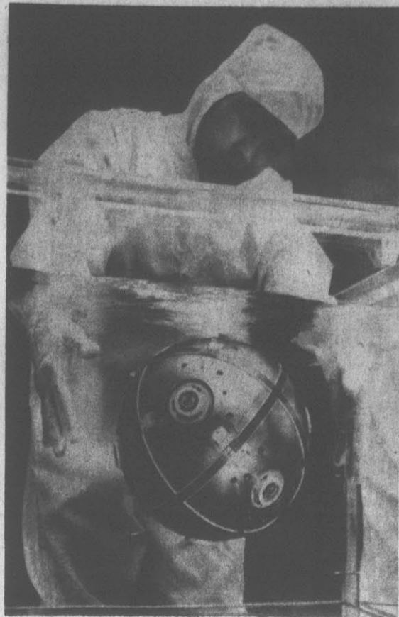
SPACE BALL. —Northrop Corporation technician tests buoyancy and balance of "floating ball" element of inertial guidance system for the U.S. Air Force's "Missile X" in the ICBM program. Ball floats on layer of special fluid in the missile to protect instruments in the "ball" from vibrations and temperature. (AP Laserphoto)
