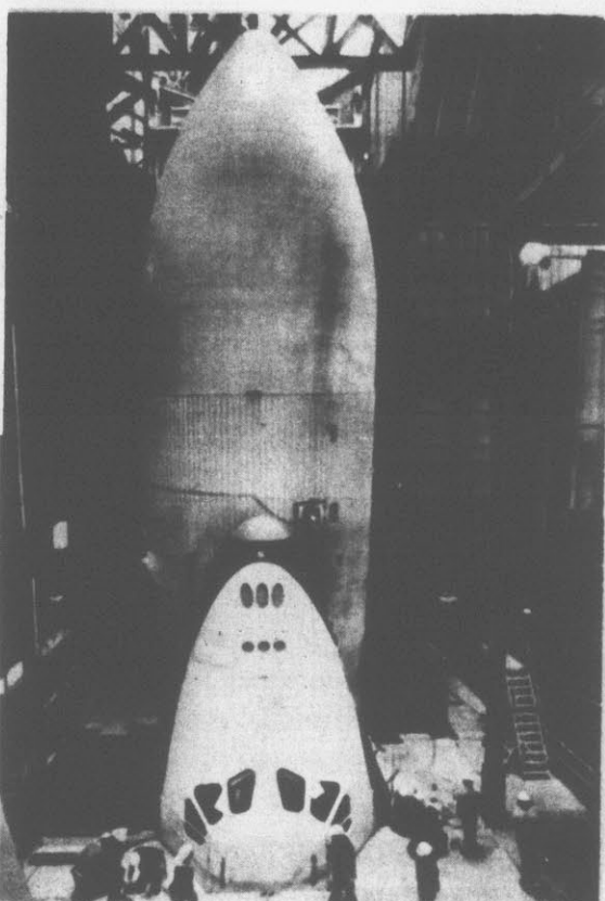
MATED — The nose of the space shuttle Enterprise sticks out through the work platform in the dynamic test stand at the Marshall Space Flight Center in Alabama. The Enterprise and its external tank are being prepared for tests that will simulate vibrations of launch. It is the first time that the orbiter and tank have been joined. (AP Laserphoto)
