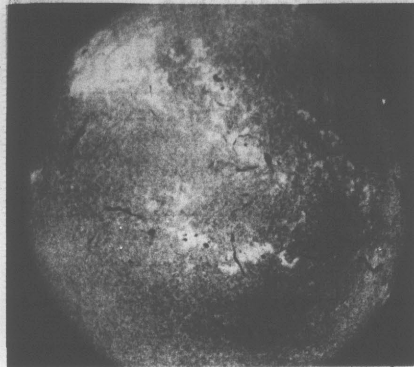
FACE OF THE SUN — An observatory photo shows the look of the sun's outer layer during a period of solar flares. The bright spot at the upper left is thousands of times larger than Earth.
