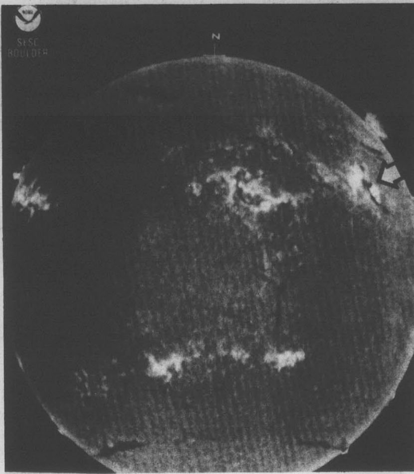
SOLAR FLARE — This photograph of the sun provided by the National Oceanic and Atmospheric Administration shows a solar flare (upper right) which is reputed to be the biggest
