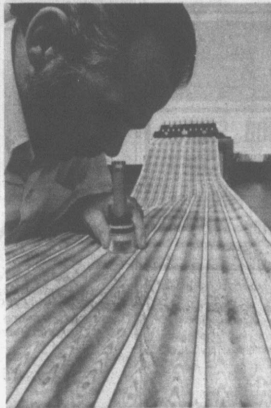
PENMANSHIP — Intricate patterns are made by 10 porous point pens undergoing an eight-hour test to determine the rate of ink usage at Gillette laboratories in Boston. George Wright, a technician, measures the width of the lines. The writing machine transcribes figure-8s — 2,500 feet of them, before the average test pen ran dry. (AP Laserphoto)
