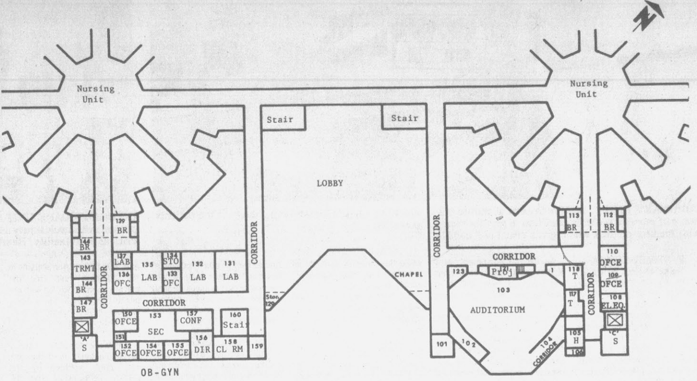
FIRST FLOOR PLAN 1/32" = 1'-0"
