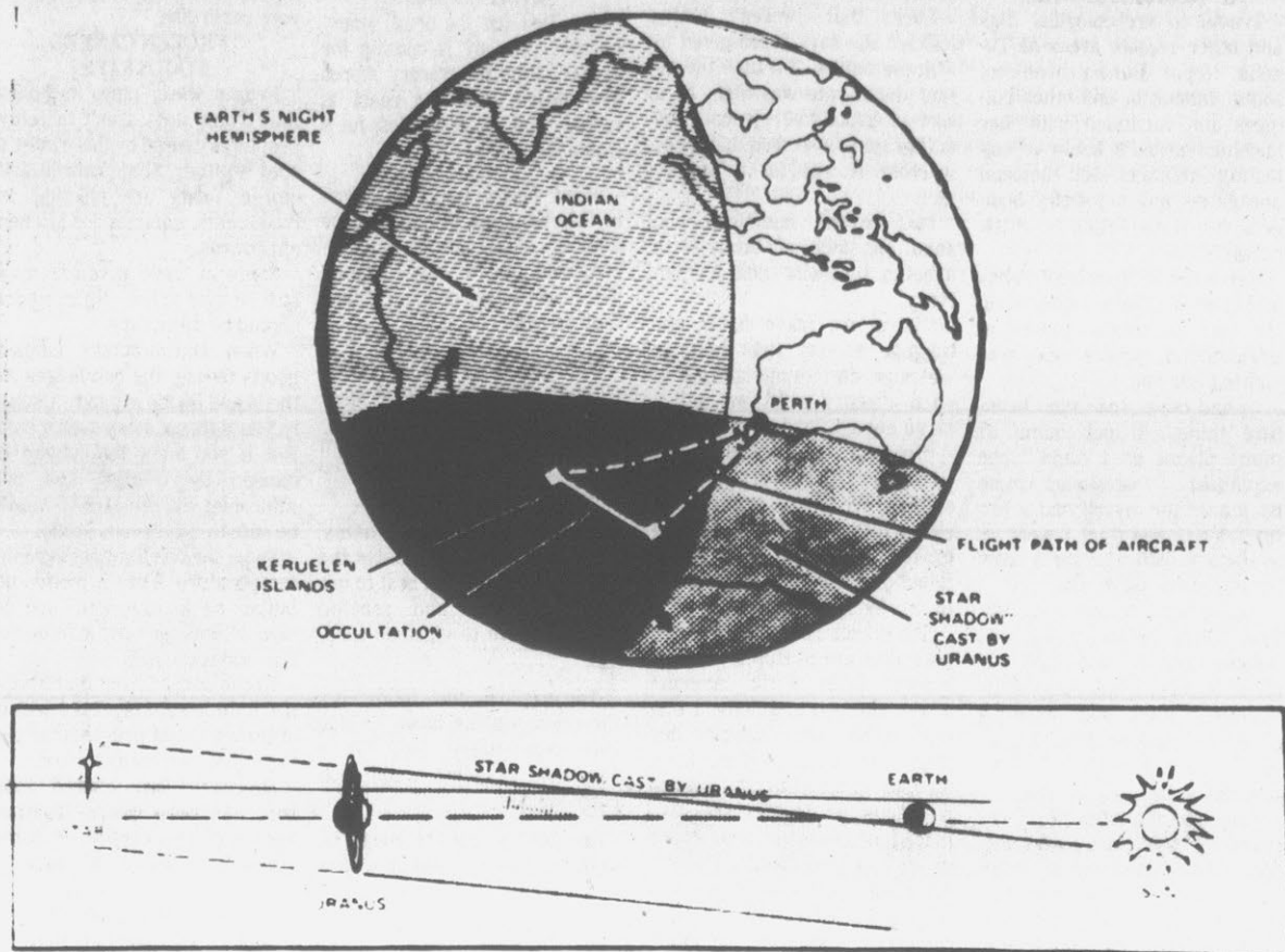
URANUS' RINGS DISCOVERED — NASA officials released this diagram in connection with announcement that rings orbiting the planet Uranus, the first major structure in the solar system to be found since
