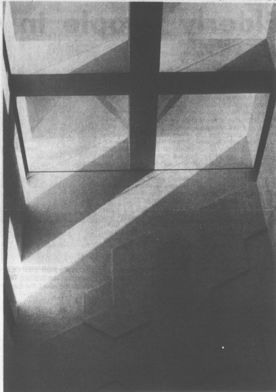
A THREE STORY HIGH SKYLIGHT — casts shadows on the sculpted walls of the rectangular open well above the main entry lobby.
