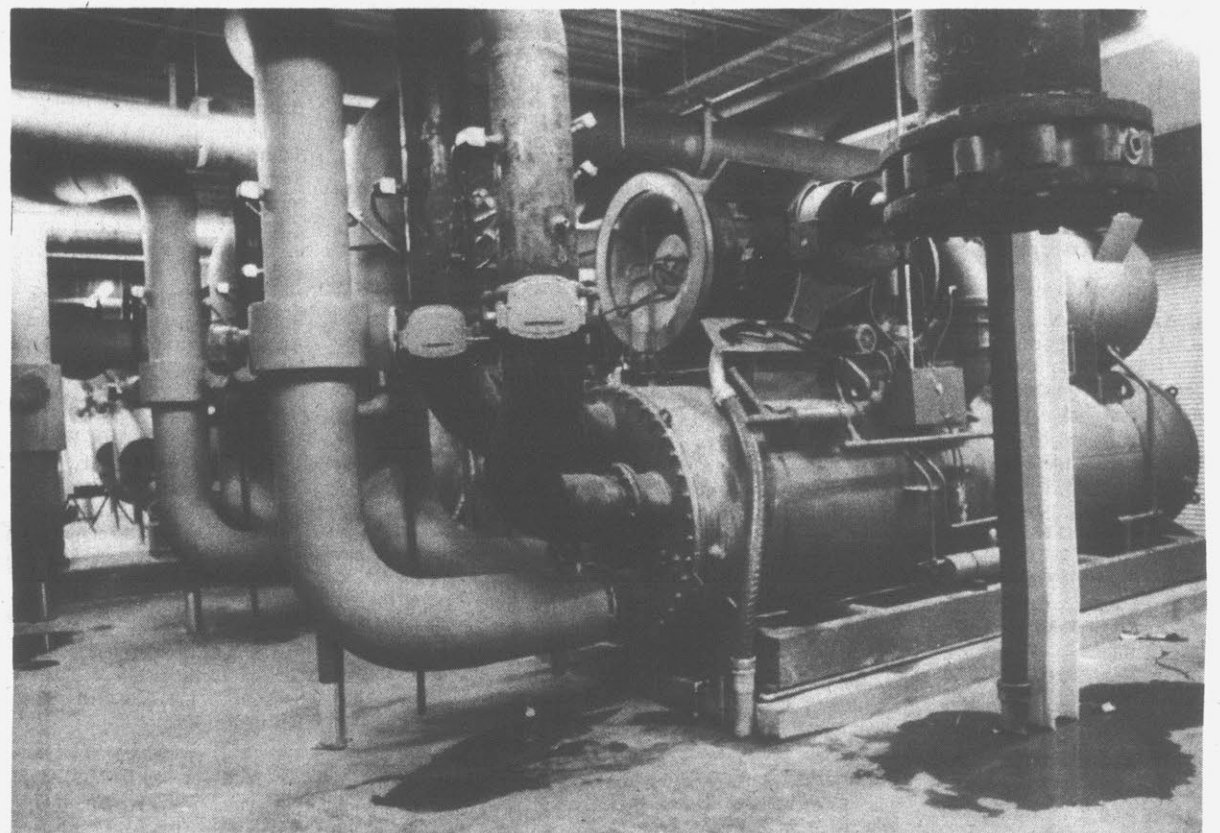
CHILLING UNITS... Large centrifugal chillers are used for chilling water to be distributed throughout the building.
