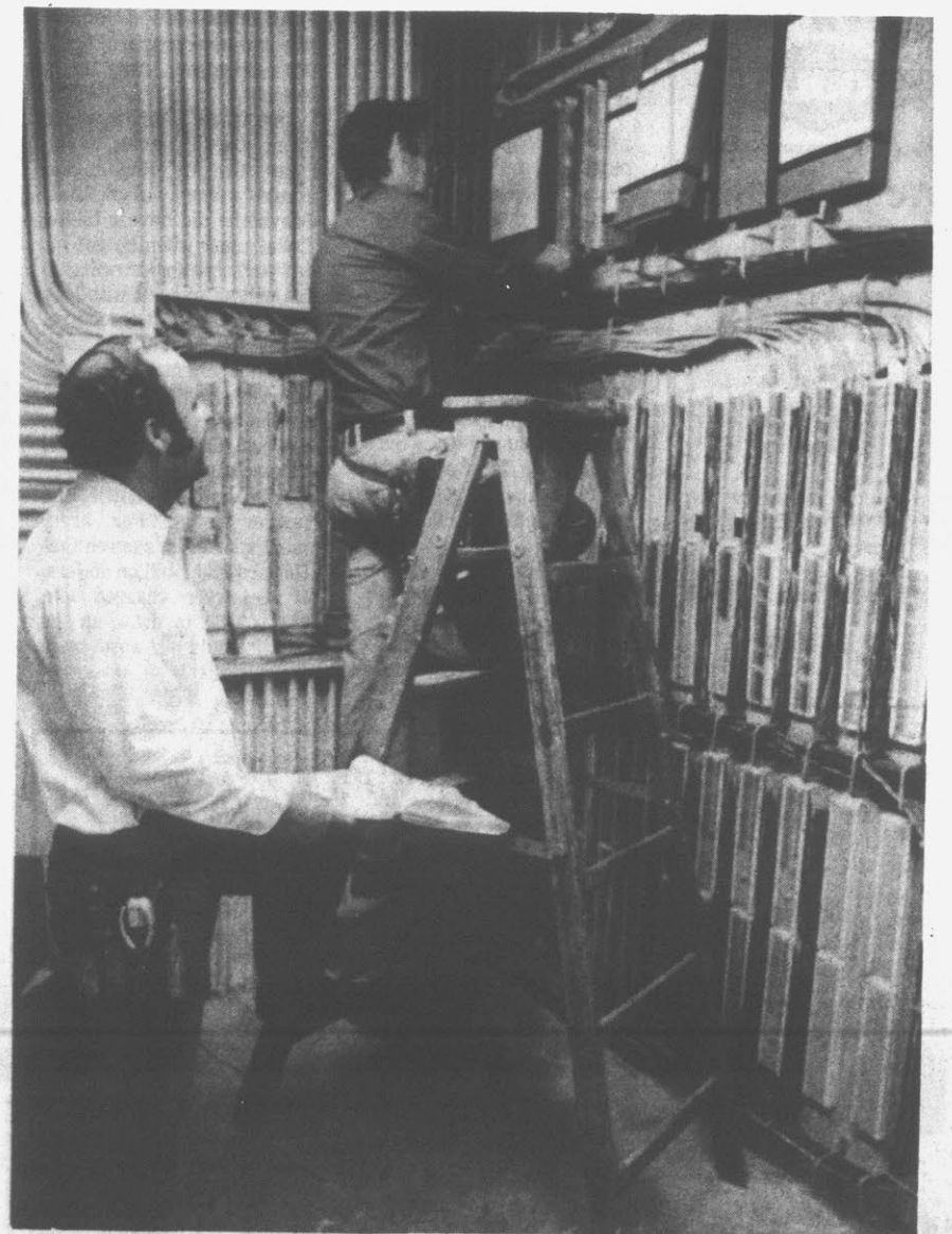
TELEPHONE EQUIPMENT... No building would be complete without communication. Telephone installers, Dewey Robinson, left, and Joseph Lamb, install equipment in one of the many terminal rooms in the building. There will be approximately 411 telephones in the facility.
