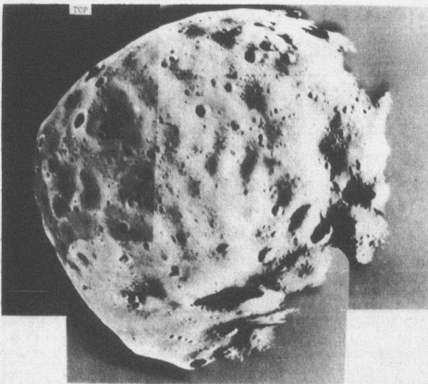
MARS' INNER SATELLITE — This photo mosaic shows Mars' inner satellite, Phobos, as photographed Feb. 18 by Viking Orbiter I at an elevation of 300 miles. As seen here, Phobos is about 75 per cent illuminated and about 13 miles across and 11.8 miles from top to bottom. The south pole is within the large crater, Hall, at bottom center where pictures overlap. A surprising discovery has been made of what apparently resemble small rounded knolls which may be surface debris from previous impacts. (AP Wirephoto via NASA)
