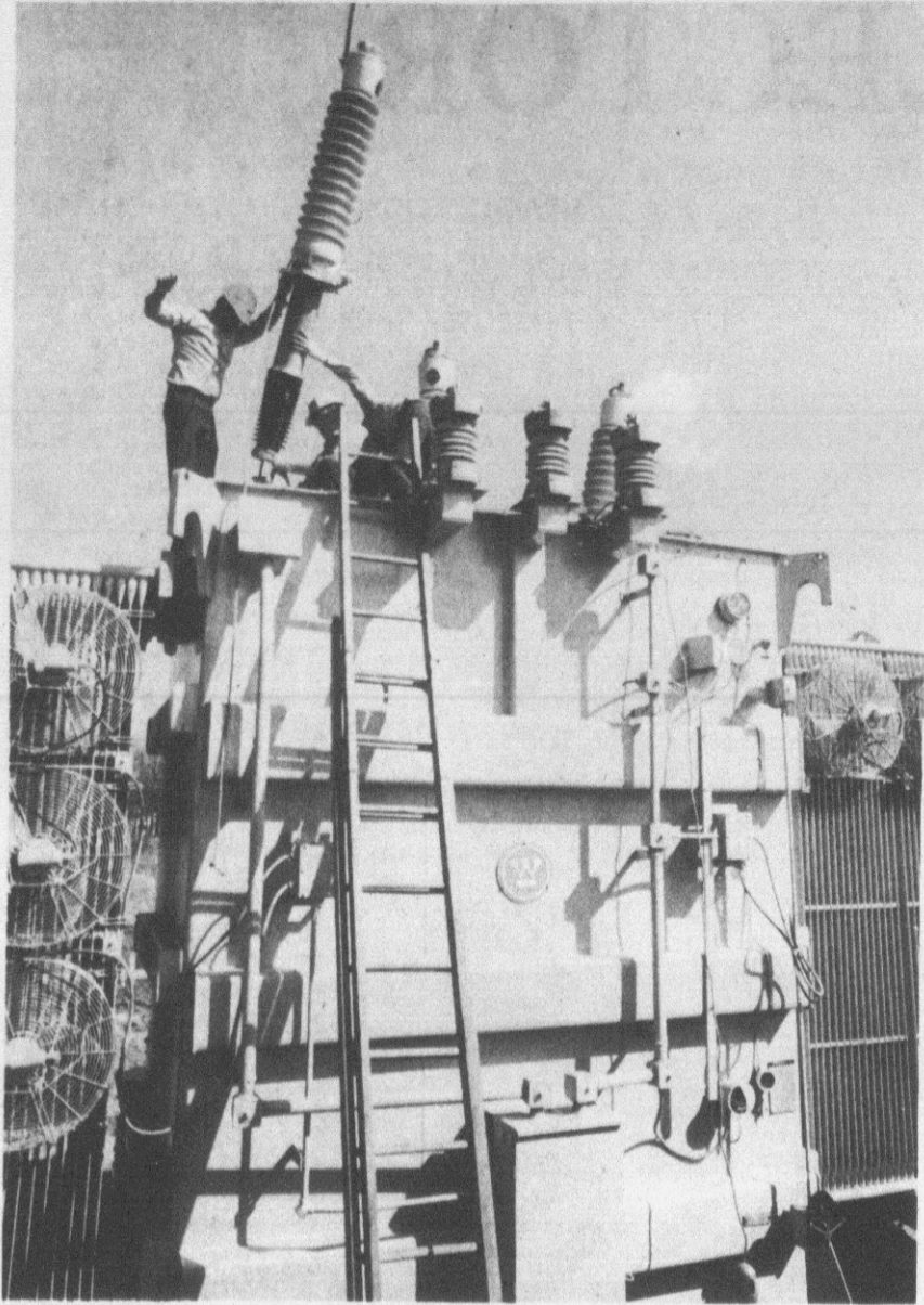
KING SIZE DIP STICK — Even though this electrical transformer is filled with 5,100 gallons of oil coolant, this isn't the dip stick. Instead it's an electrical bushing to be lowered into the transformer. The unit is part of a renovation project at the southside substation on Greenville
