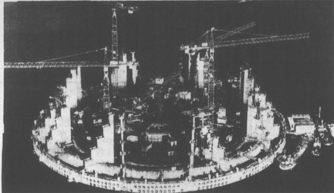
GIANT OIL PLATFORM —The huge Ninian Central platform being built for Chevron Oil's Ninian North Sea oil field is moored in Loch Carron, Scotland, with its massive base structure showing above water. When completed it will weigh over 400,000 tons. The indents on the side walls help resist sea pressure. (AP Wirephoto)
