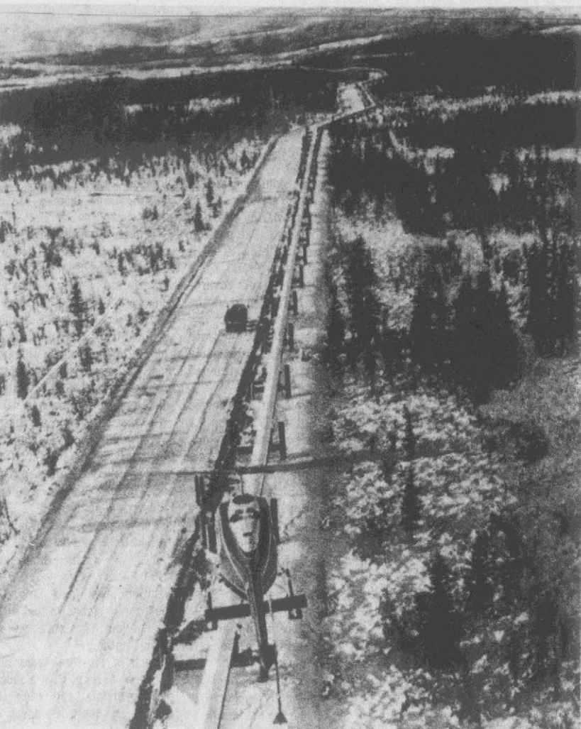
FLYING THERMOMETER — Special heat-sensing equipment inside this helicopter will show weather special heat pipes inside the vertical supports of the trans-Alaska pipeline are working. The pipes are designed to keep Alaska's frozen land frozen. (AP Wirephoto)
