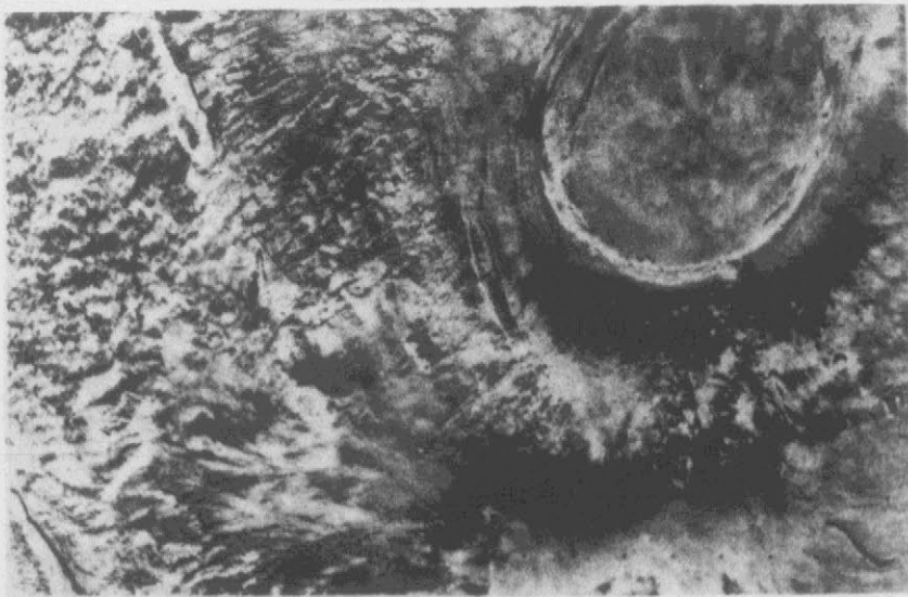
17-MILE HIGH MARTIAN CRATER —This montage of four photos taken by Viking Orbiter shows one of the enormous volcanoes in the Tharsis region near the equator on Mars. The volcanic crater Arsia Mons is 62 miles in
