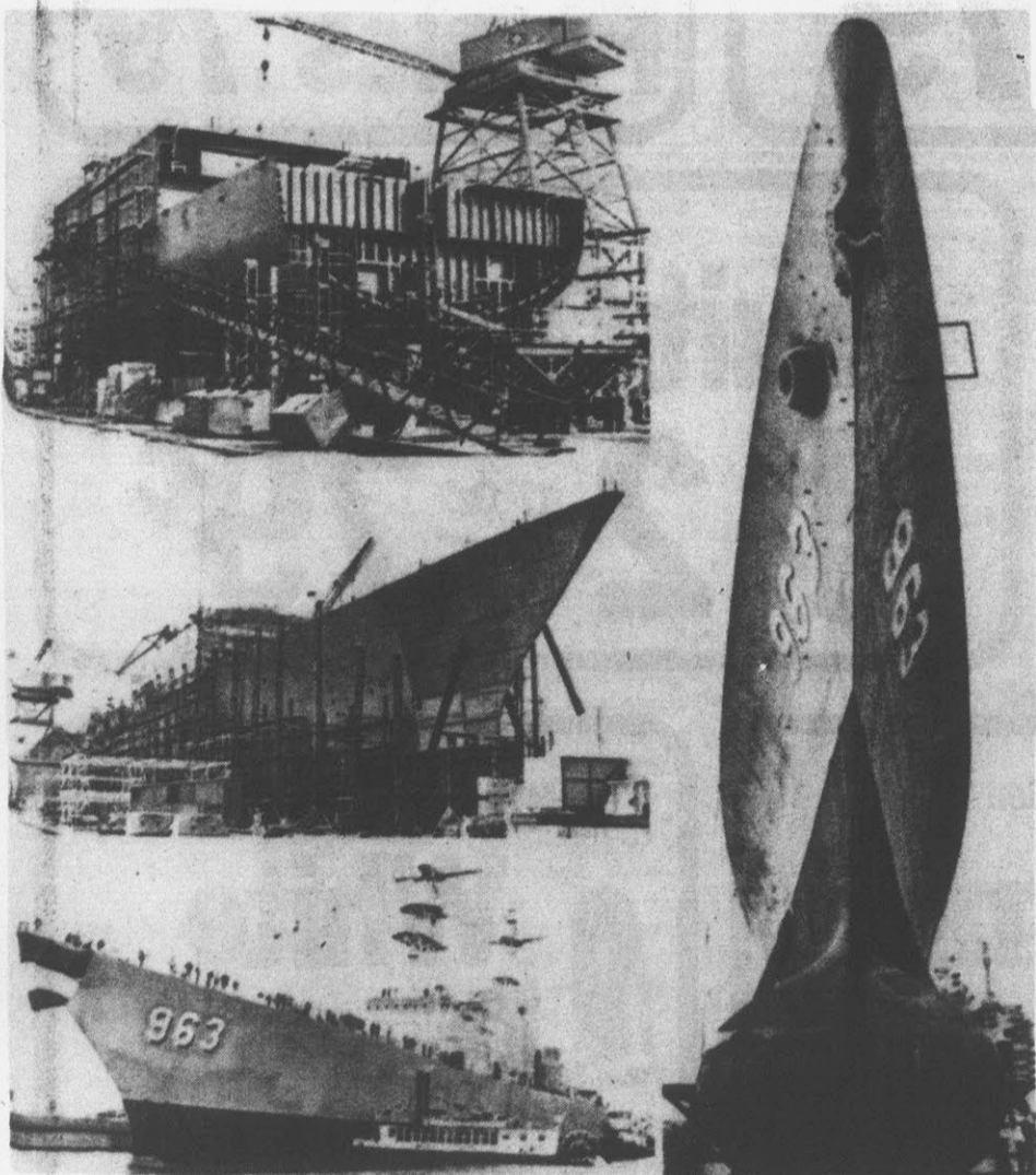
BUILDING THE SPRUANCE — These series of pictures shows the Navy destroyer Spruance in early stages of modular construction and upon completion at Ingalls Shipbuilding Division at Pascagoula, Miss. The photo at right indicates the sleek lines of the extremely fast ship, one of 30 being constructed at Ingalls. (AP Wirephoto)
