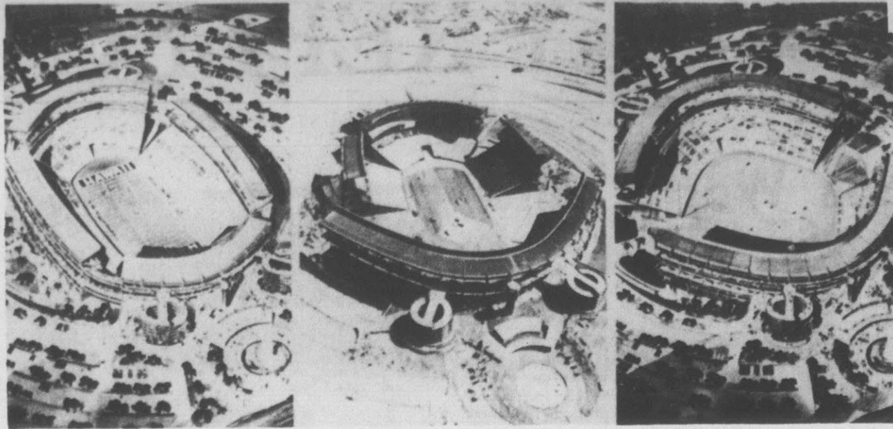
CONVERTIBLE STADIUM —The new Aloha Stadium in Honolulu was built to provide ideal accommodations for both football and baseball. However, the method chosen to achieve that goal was so unusual that the architect had to post $1 million bond in case it didn't work. Four sections of the stadium, each weighing 14
