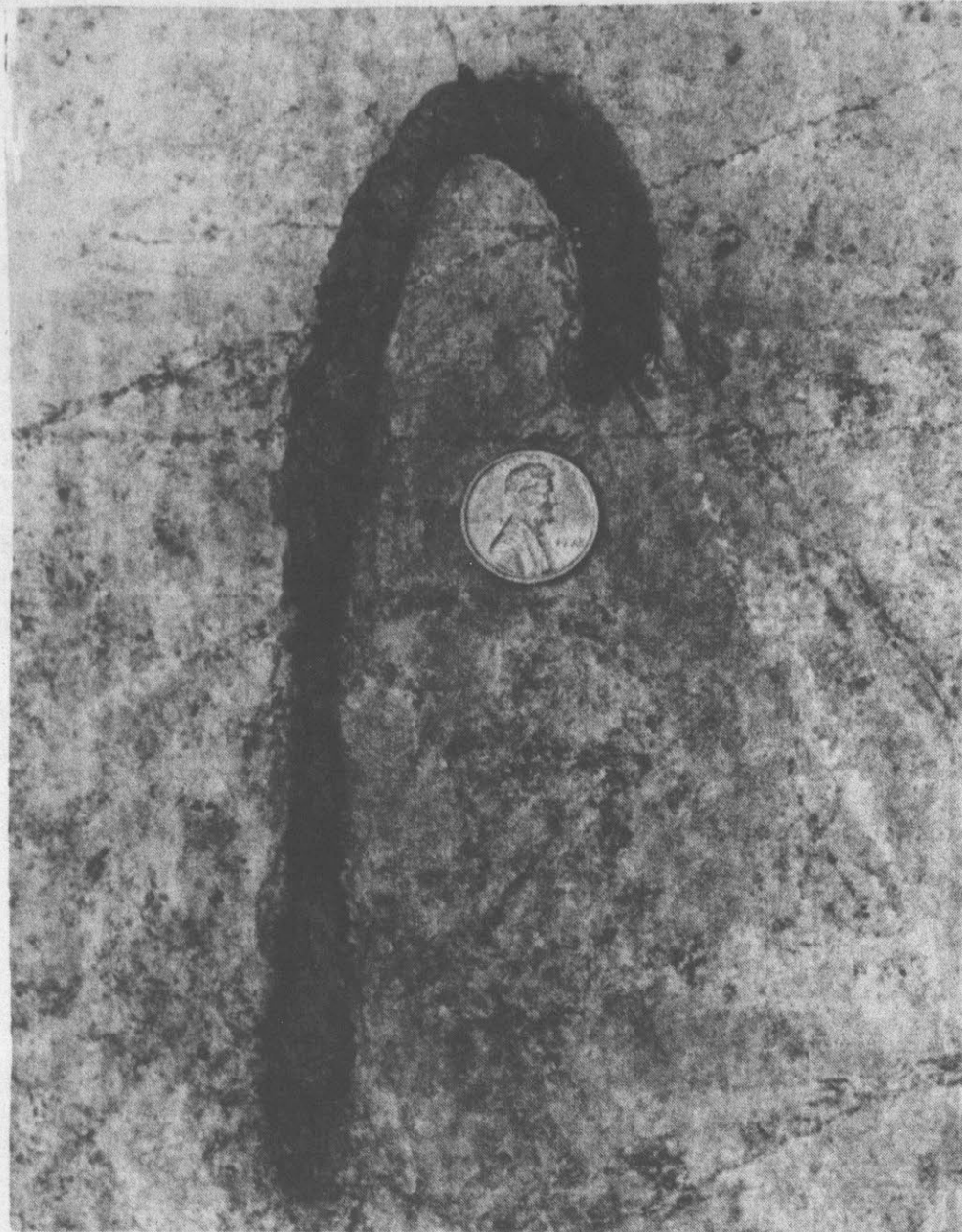
OLDEST FOSSIL —This fossil of a marine worm measuring about 9 inches is one of the several dating back more than 620 million years, according to Virginia Polytechnic Institute geologists who found them in a rock slab on the
