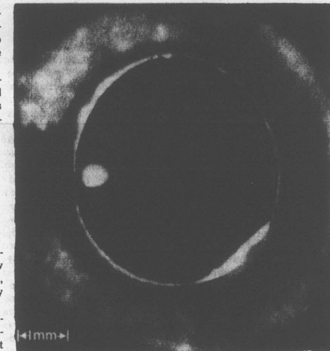
LIQUID ELECTRICITY—Physicists at the University of California in Berkeley have made the first photograph showing electricity in liquid form. The photo shows what scientists call an "electron-hole drop" created by laser light in a small circular crystal of extremely cold germanium. The bright spot at the center left is the flowing infrared image of the drop. The bright ring is infrared light scattered from the crystal edge. The drop actually measures about one-thirtieth of an inch in diameter and is estimated to contain some ten thousand billion electrical charges. (AP Wirephoto)
