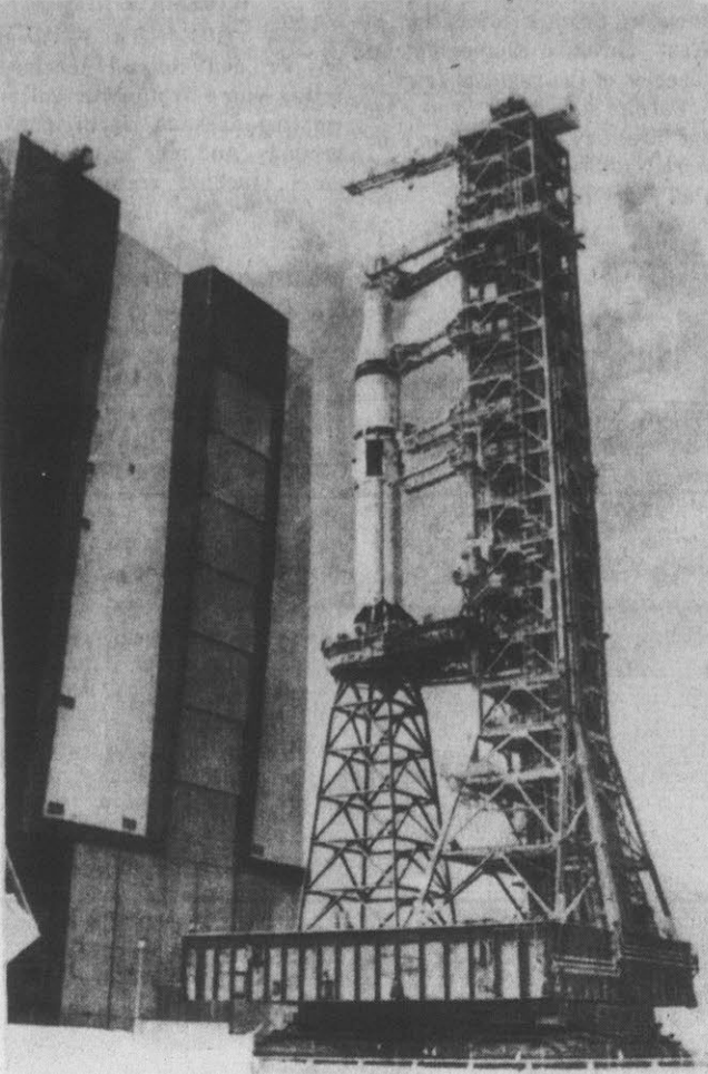
VIBRATION TEST —Scientists at Cape Canaveral Sunday staged a vibration test to see if the 80-foot-tall lightning mast atop the Saturn 1B mobile launcher can stand the .8 MPH speed to the complex 39B pad. This rocket will be used in July's Apollo-Soyuz flight. (AP Wirephoto)
