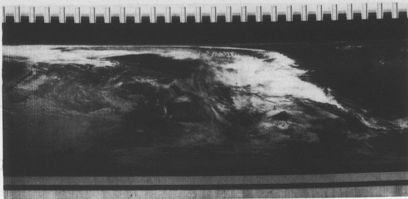
WEATHER PICTURE FROM 700 MILES ABOVE EARTH . . . This is one of the photographs Dail was able to receive from the Improved Tiros Operational Satellite. The bottom section of the photo is for in-
