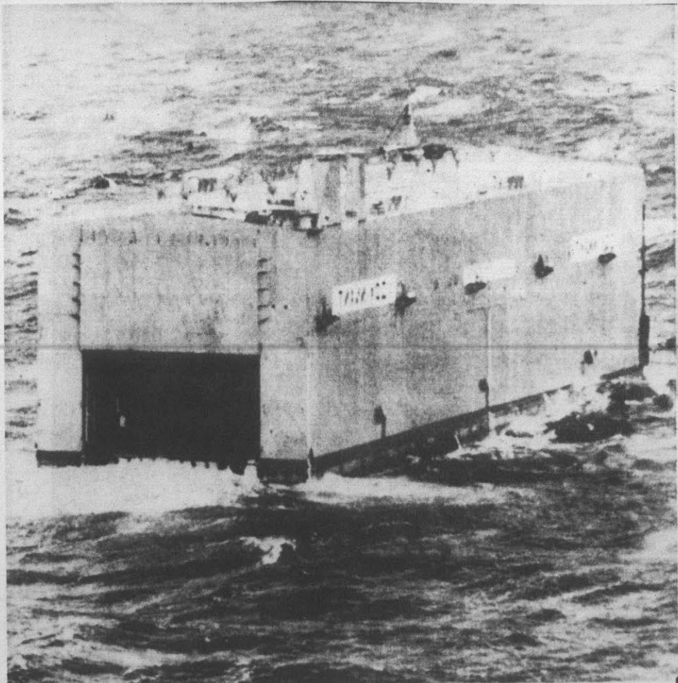
FLOATING DOCK —Sighted in the North Sea by a British Royal Air Force Nimrod reconnaissance aircraft was this latest addition to the Russian Navy—a vast mobile floating dock designed to cut the time submarines have to spend off station for a refit. The dock is thought to take two of the largest nuclear powered submarines at a time,
