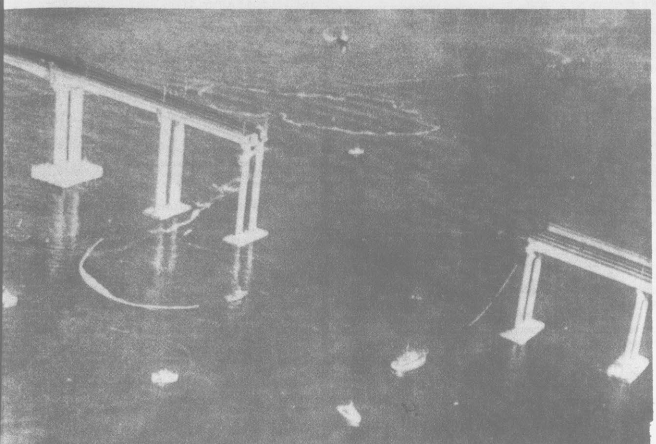
BRIDGE COLLAPSES—The Tasman Bridge across the Derwent River at Hobart, on the Australian island state of Tasmania, is shown after it was struck Sunday evening by the freighter Lake Illawarra, causing the collapse of a bridge section on the freighter
