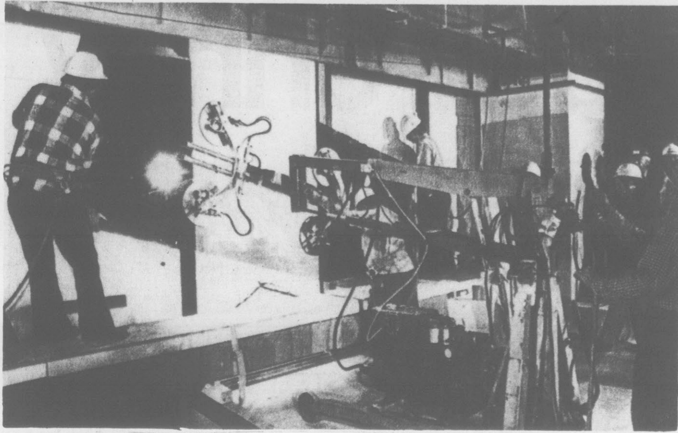
NEW GLASS FOR SKYSCRAPER — Workmen use a suction device to move a 400-pound glass pane into place on the 58th floor of Boston's John Hancock Building. The new structure was plagued with falling windows which had to be covered with plywood until
