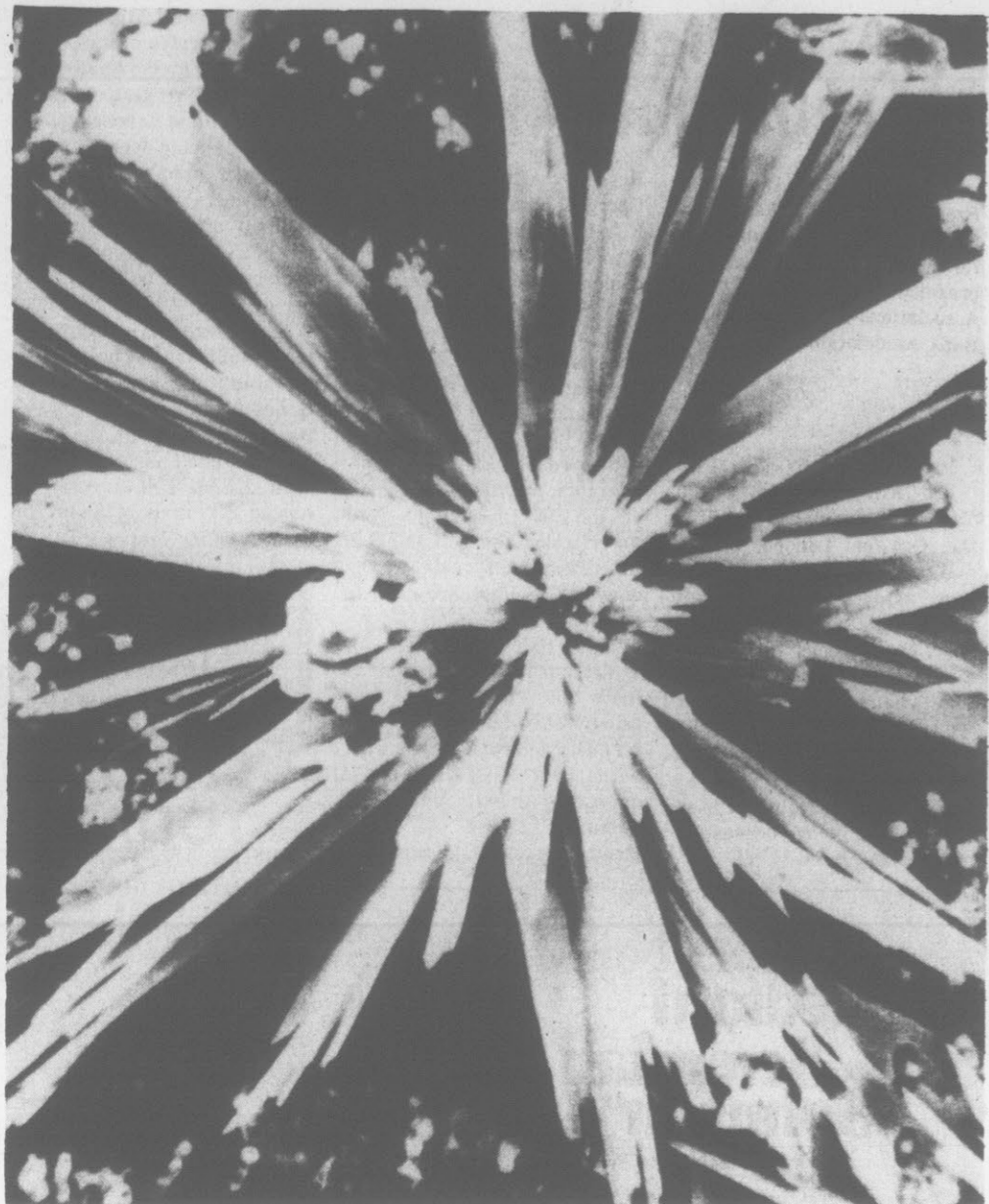
CRYSTAL CHRYSANTHEMUM — What appears like a chrysanthemum is actually a lead crystal magnified 2,000 times and produced by chemical action on the negative electrode of a lead acid battery. Photograph was taken with a
