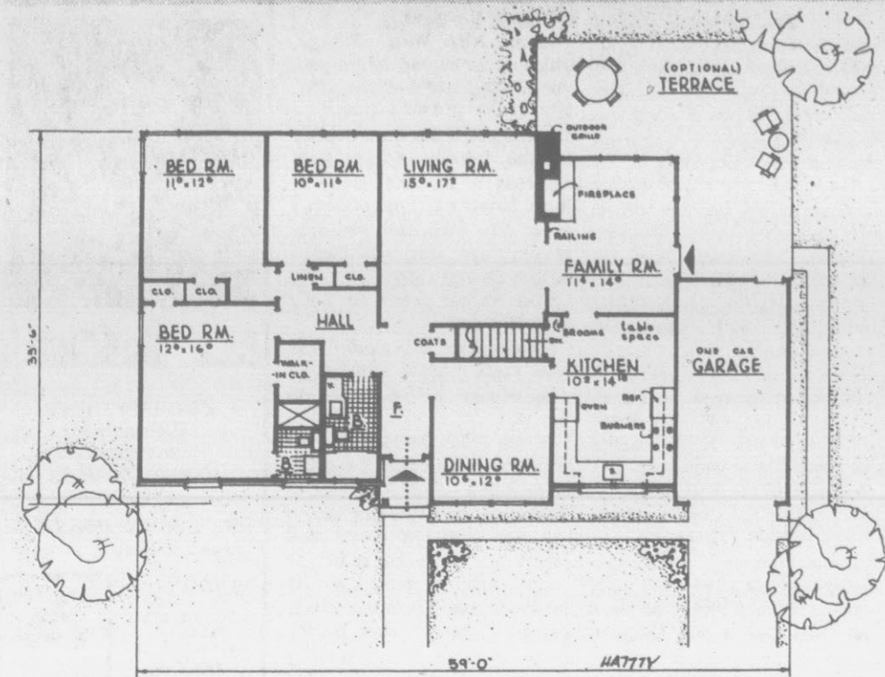
SMARTLY STYLED in shingle and brick, this ranch home, Plan HA777Y, combines good taste with common-sense planning. A covered entry leads to a large foyer which has a convenient coat closet within easy reach. The center hall from this point leads to all areas. There are three well-ventilated bedrooms, with walk-in closet and private bath for the master. The living room has a long, unbroken wall for variety of furniture placement. The family room has a fireplace and a convenient entrance to the kitchen. The kitchen's arrangement is U-shape and there is table space and a broom closet at one end. Architect of the 1,536-square-foot house is Herman H. York, 90-04 161st St., Jamaica, N.Y. 11432. Anyone wishing to know the price of the blueprint can write to him.
