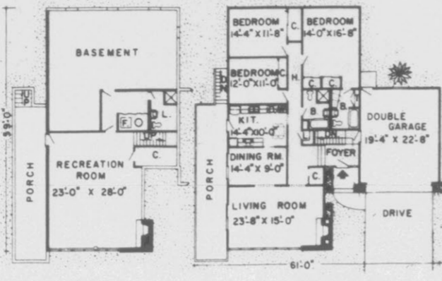
Size: 1,763 sq. ft. first floor; 1,763 sq. ft. basement; 459 sq. ft. garage. Over-all dimensions: 61 ft. by 59 ft.
