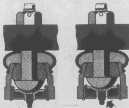
Ball joint wear indicators. Ball joints are an important part of your car. These wear indicators show if they need to be replaced.
