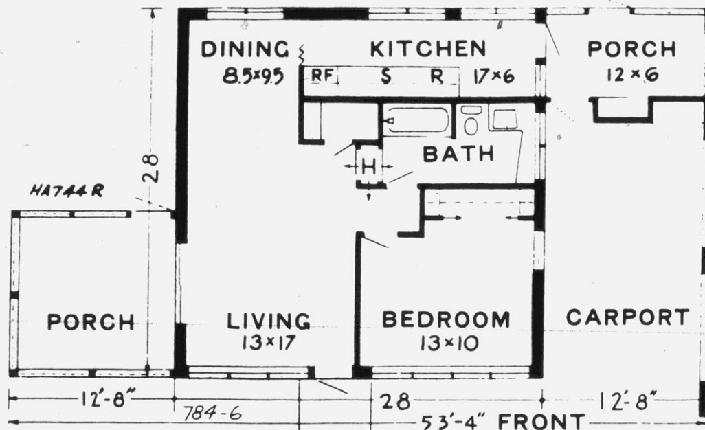
THE GENTLY SLOPING saddle roof of Plan HA744R makes the house look much larger than it really is. The 12 by 12 screen porch extends the living room, via a sliding glass door. The dining area is handy to the kitchen. And the kitchen has a breakfast nook, as well as a door to a back porch, also suitable for outdoor eating. There are 784 square feet in this home, designed by Jan Reiner, 1000 52nd St. North, St. Petersburg, Fla. 33710.
