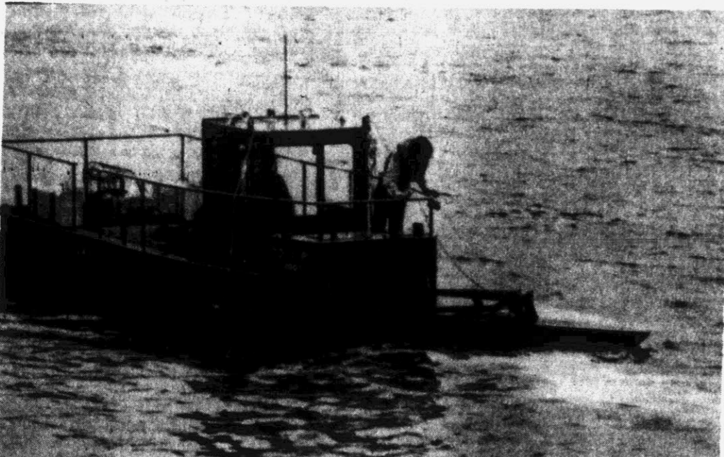
OIL SPILL CLEANER — The U.S. Navy demonstrates its new Skimmer Workboat designed to clean up oil spills in harbors and near shore areas in Boston Harbor. Dubbed the JBF-DIP 3001, the 25-foot craft cuts a 13-foot swath through an oil slick and can harvest 2,000 gallons of oil in an hour. The craft shown here is intended for use at the Puget Sound Shipyard in Bremerton, Wash. (AP Wirephoto)
