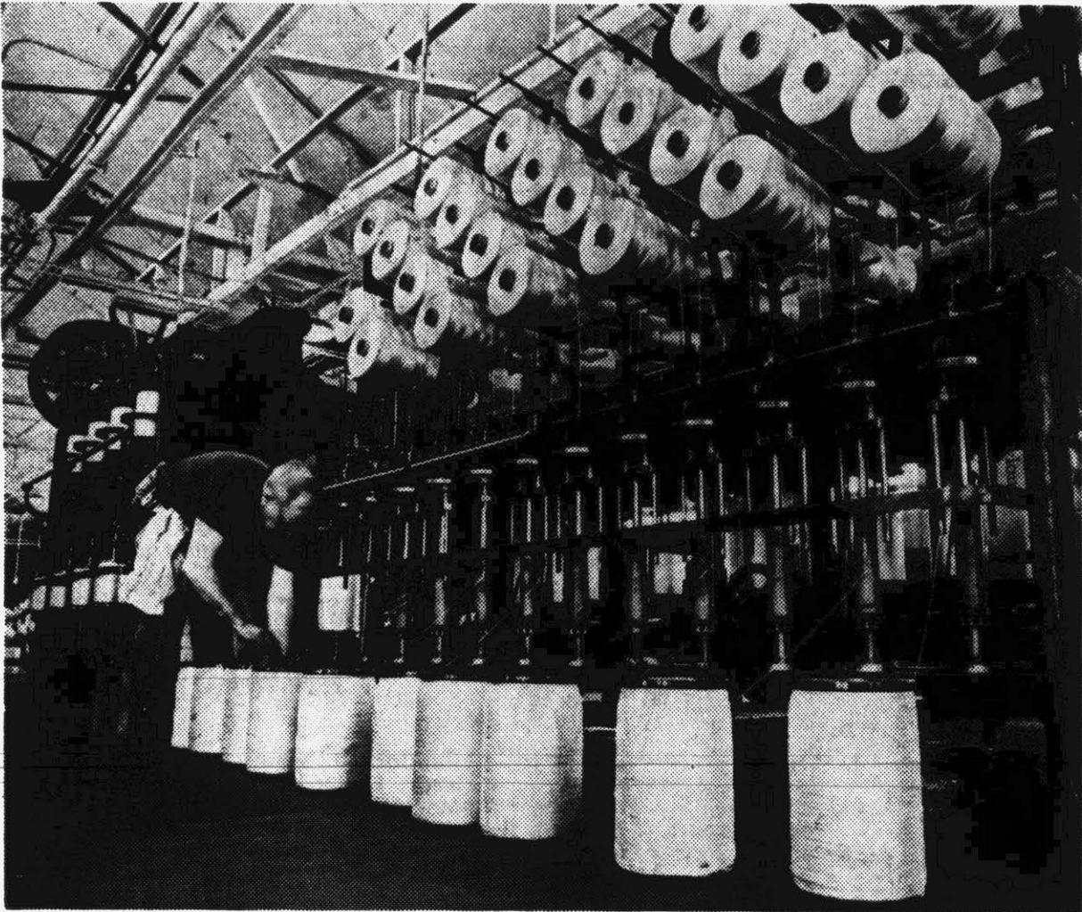
The machines above are some of the Ropewalk's oldest, still in use after 35 years. The modern ones below, two years old, spin nylon fibers into cord.
