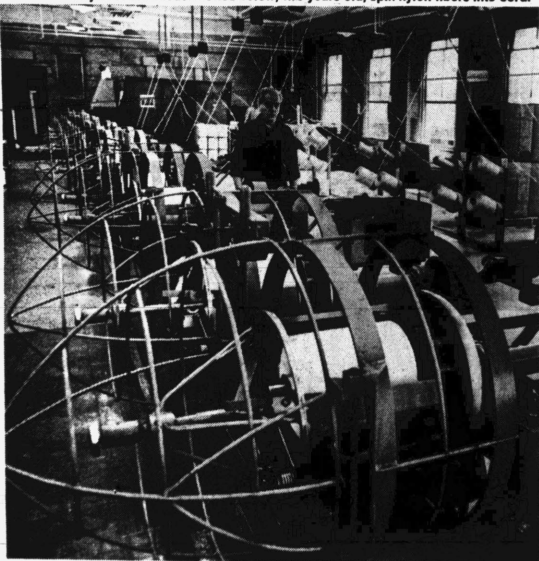
The machines above are some of the Ropewalk's oldest, still in use after 35 years. The modern ones below, two years old, spin nylon fibers into cord.
