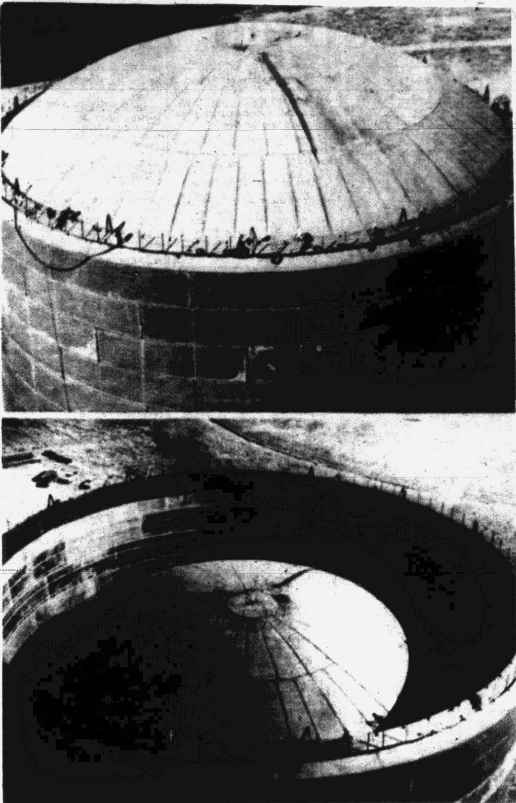
ROOF RAISED BY AIR PRESSURE — The 100-ton steel top to Atlanta Gas Light Company's new liquefied natural gas tank at Riverdale, Ga., was constructed on the floor of the tank and then raised 142 feet to the top by air pressure. Note the workmen on the rim of the tank. The new tank will hold enough gas to provide the residential requirements for an entire year for a city of 30,000. (AP Wirephoto)
