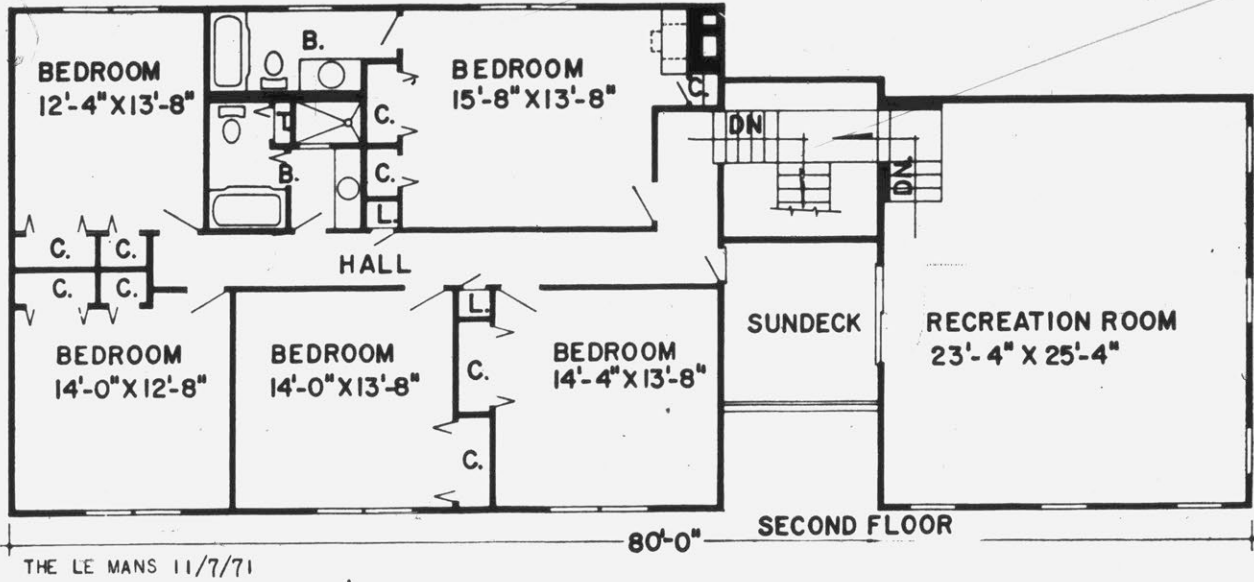
A RUSTIC BEAUTY — The Le Mans, a six-bedroom, two-story home is tailored to the needs of a large family. There are three and a half baths, a living room, dining room, kitchen with dining space, laundry room, foyer, large recreation room above the double garage with adjoining sundeck, and full basement.
