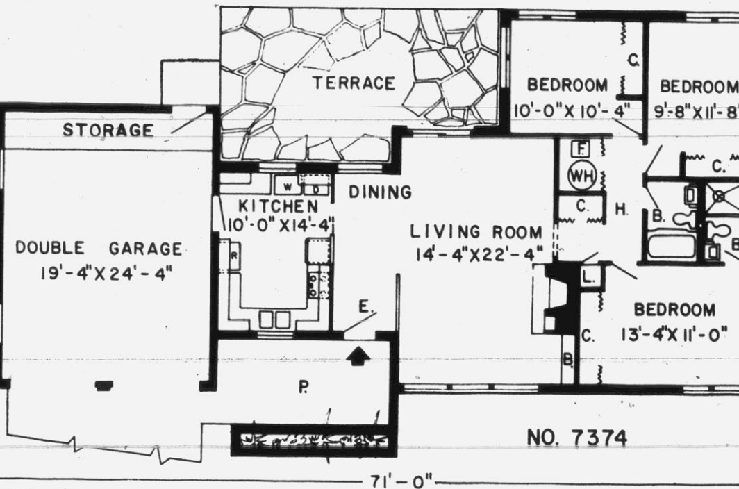
A SNUG HAVEN — The Cassadaga would make a snug home for a modern family. There are three bedrooms, two baths, a living room-dining room area, modern kitchen and double garage. Plans call for one-story construction of concrete masonry units.
