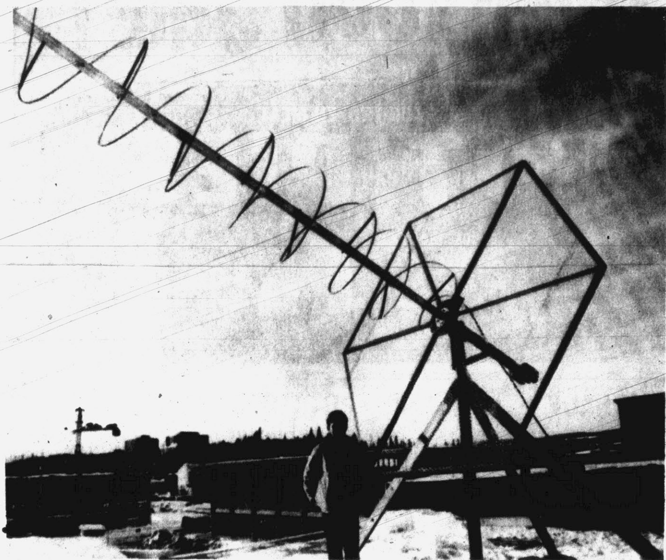
THIS HELICAL ANTENNA, and taxicab radios, may bring two-way radio communications to remote
