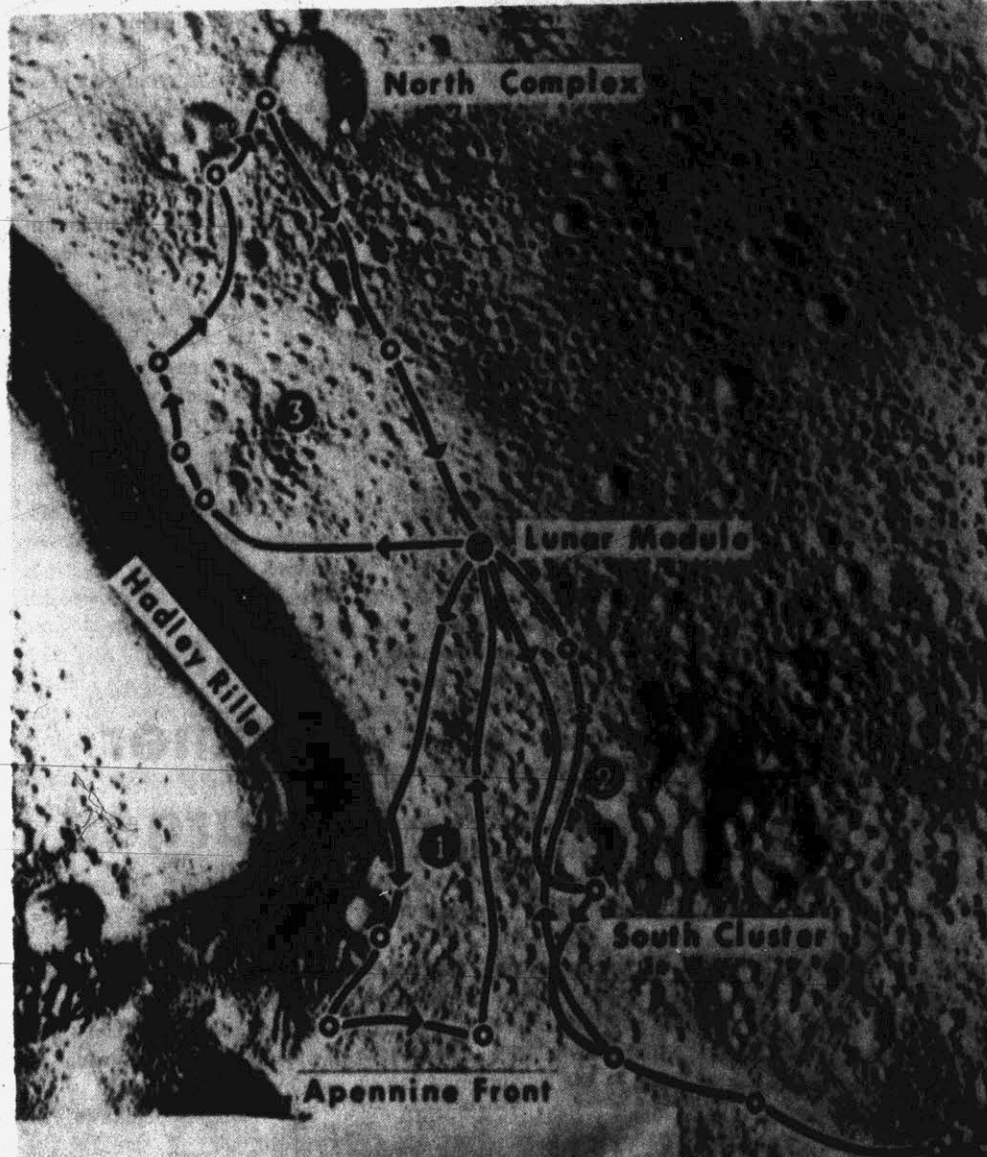
MOON EXPLORATIONS — Relief map diagram locates the three explorations Apollo 15 astronauts David R. Scott and James B. Irwin will take on their three days on the lunar surface. Saturday's trip (1), was to the Apennine Front. Sunday's trip (2), along the South Cluster. Monday's trip (3), along the Hadley Rille and the North Complex. (AP Wirephoto)
