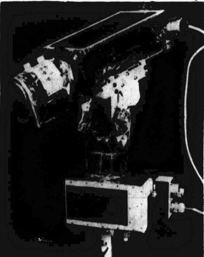
COLOR CAMERA — This is a close-up of the flight model of the color television camera and television control unit which will be used on the Apollo 15 lunar landing mission. The camera is for lunar surface use and will be operated from three different positions — mounted on the Lunar Module's Modular Equipment Stowage Assembly; mounted on a tripod and connected to the LM by a 100-foot cable; and installed in the Lunar Roving Vehicle. (AP Wirephoto)
