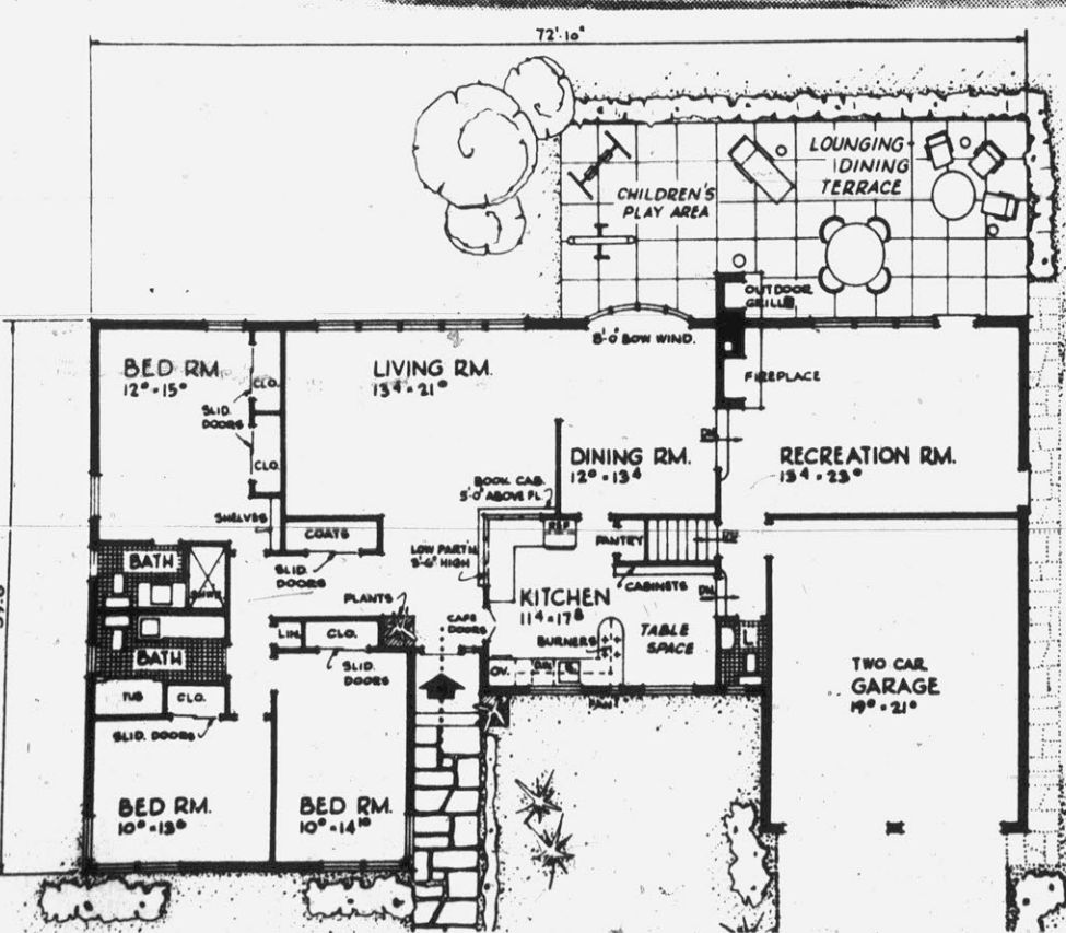
MODIFIED RANCH: This impressive plan has seven rooms with two baths, a lavatory that separates the kitchen and the two-car garage, and a full basement. A recreation room with a fireplace leads to an outdoor terrace and grill. This home measures 1,987 square feet, plus garage. Plan HA678Y was designed by architect Herman H. York, 90-04 161st Street, Jamaica, N.Y., 11432.
