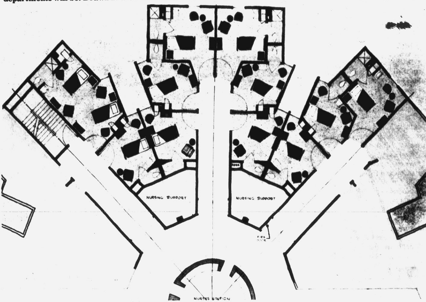
HALF OF ONE FLOOR . . . of a nursing tower is shown. Note the spaciousness of each room, that each has a window and a toilet and lavatory, and the closeness of the nursing support rooms to the nurses' station which is the hub.
